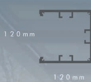
Poteau
